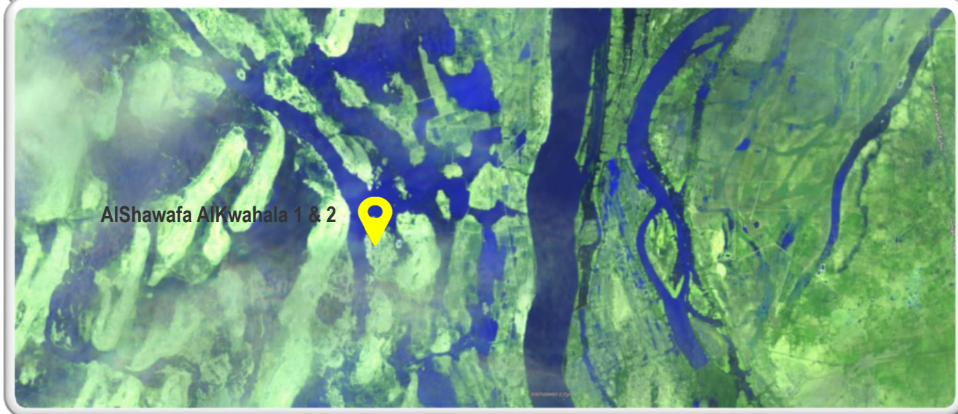
Sentinel-2 acquired on 21 Aug 2019
