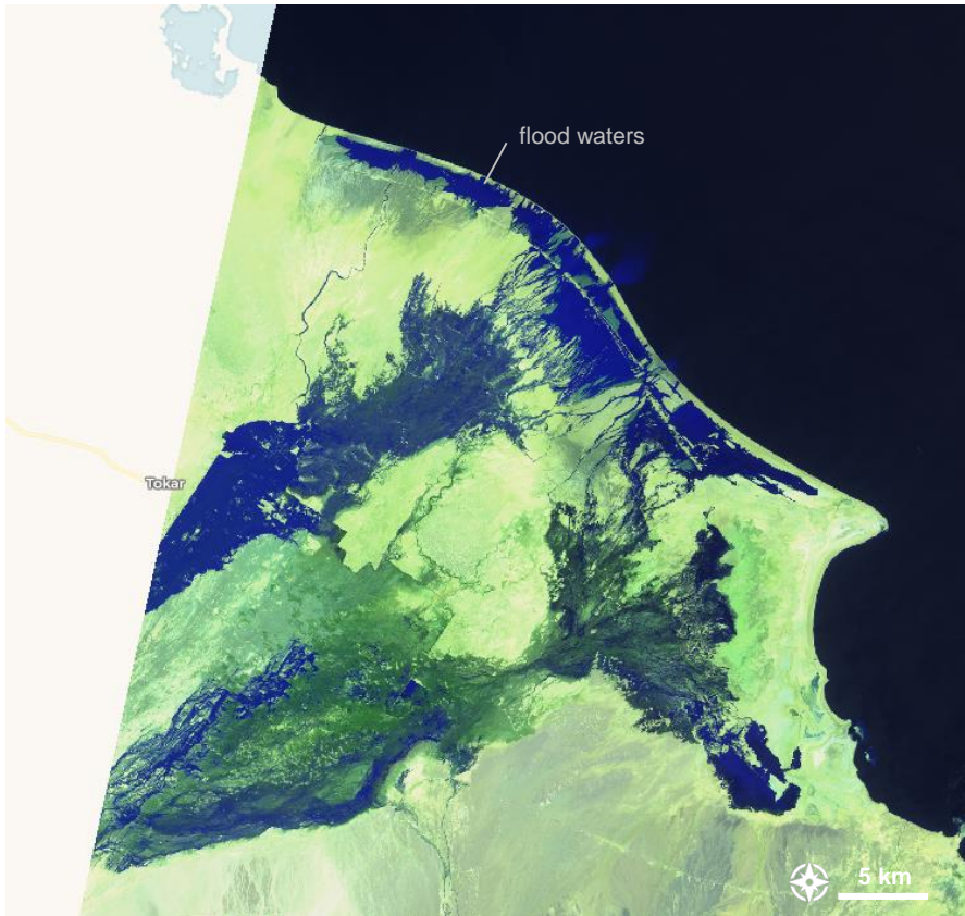
Sentinel-2 false color composite acquired on 15 Aug 2019
