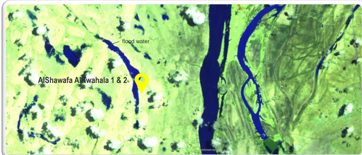
Sentinel-2 acquired on 6 Aug 2019
